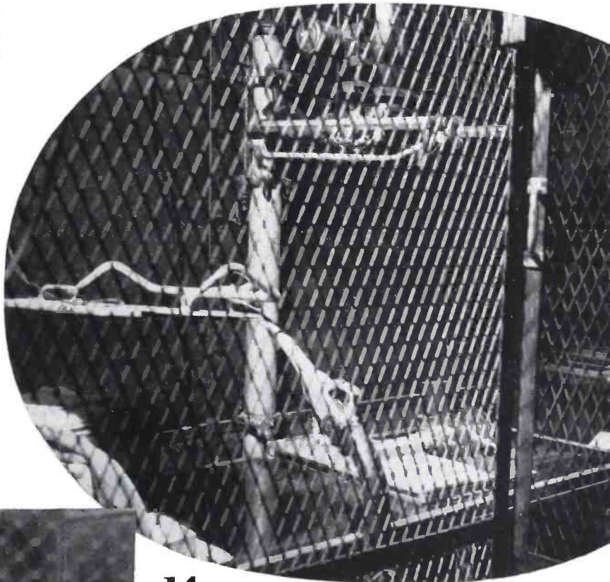
Spot-knocking or high-voltage treating the rebuilt tube after its exhaust. This burns off any infinitesimal points on the internal parts and assists in eliminating any minute traces of gas (air) which might be occluded internally. A controllable voltage of from 25,000 to 50,000 volts is applied through a current-limiting resistance. Tube pictured through safety glass has good vacuum as is evidenced by high voltage arc across outside of glass envelope although the external distance is many times the internal element spacing.
