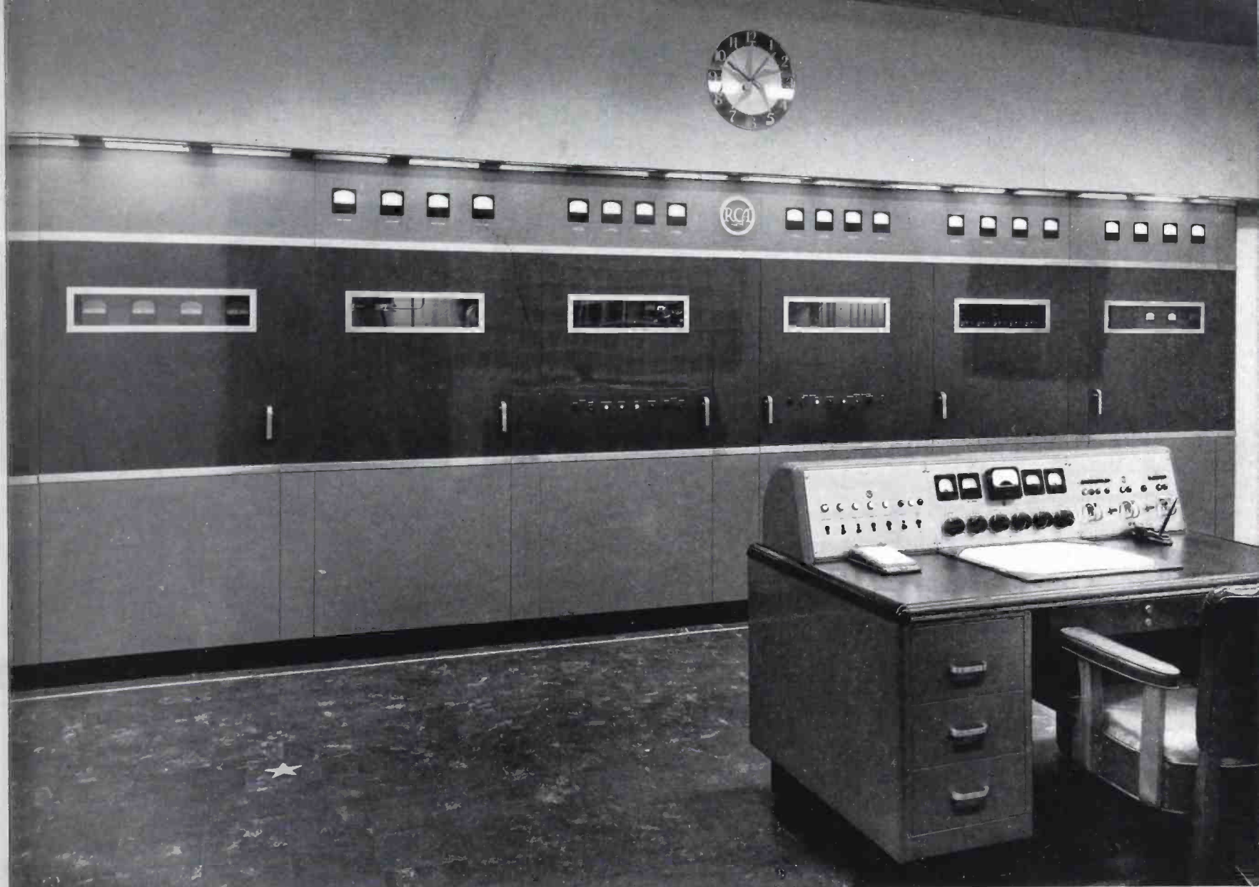
KMPC TRANSMITTER ROOM —The 10-E transmitter, the phasing equipment for the three-tower antenna array, and the speech input and monitoring equipment are all mounted behind the single “unified-front” type enclosure shown above. The operator’s console and a monitoring speaker mounted in the ceiling are the only other items of equipment in the transmitter room. The extra panel units which make this ultra-streamlined installation possible are optional accessories with the 5-E and 10-E transmitters.
