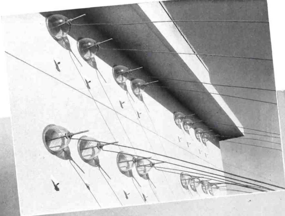
TRANSMISSION LINES —Each of Radio Nacional's eight antennas is fed by a transmission line from the main building. This interesting view shows these lines as they emerge from the building.
