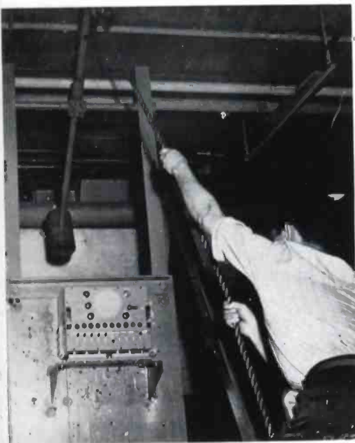
GUN RECOIL PUNISHMENT is dealt out by the repeated blows of a solid steel sledge-hammer in this so-called "shock" test. The sledge-hammer is made to deliver blows of great weight against the back of the board to which the apparatus is shown fastened.
