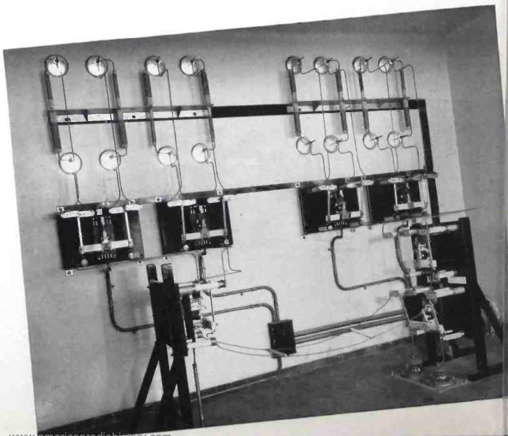
ANTENNA SWITCHING —This group of relays and switches allows the output of the transmitter to be connected to any of the eight antenna transmission lines. Switching is controlled by push-buttons in the transmitter room.
