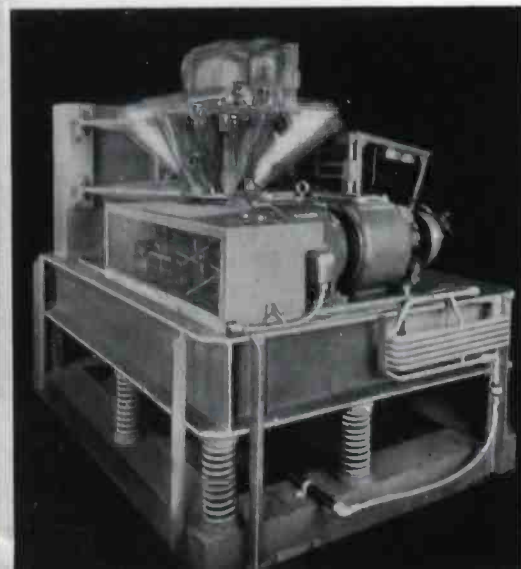
200 MILES IN A JEEP . . IN TEN SECONDS, three thousand times a minute the radio equipment atop this machine lives through an acceleration that would cause the toughest young airplane pilot to "black out" in dive bombing. In a few minutes it lives through the jars and vibrations it would receive on ten round trips from Washington to Chungking.
