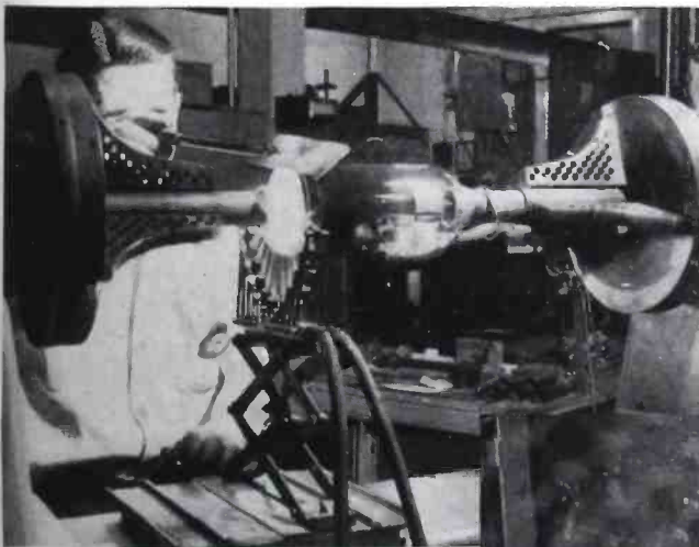
The rebuilt tube is X-rayed to make sure that all internal elements are correctly aligned. Due to safety regulations, this picture was taken through the protective grille work. The tube rests on a small table with the X-ray tube beneath it and the special camera above.
