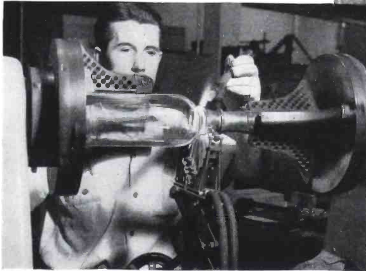
The old anode, with its new feather-edged copper cone, is sealed or welded to a new glass envelope. This large, glass-to-metal seal is made in a glass-lathe. Carefully controlled gas flames heat the rotating glass and metal parts while a skilled craftsman molds the glass around the feather-edge of the metal cone, producing an actual weld or fusion of the glass and metal. The resulting joint must be mechanically strong and vacuum-tight. The glass must be annealed carefully to eliminate any glass-strains which might later result in a crack in the glass.
