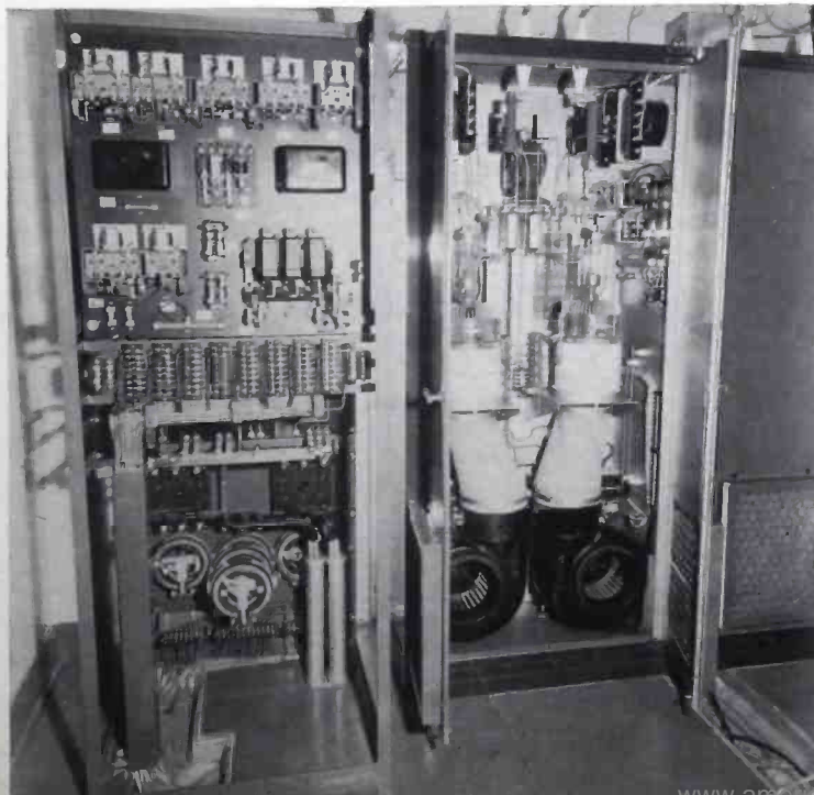
FIG. 3. Spotlessly clean equipment is one mark of a well-maintained station. Rear view of the power control unit of the 5-DX transmitter at WSYR, Syracuse.
